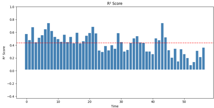
3 masking
