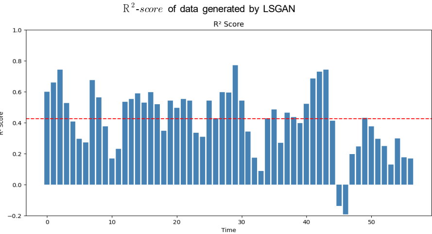
R^2 -score of data generated by masking-LSGAN
