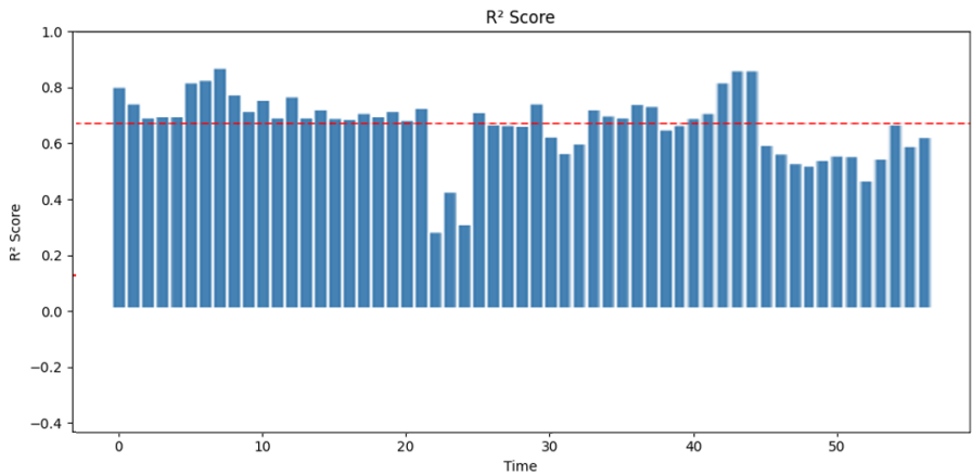
1 masking
