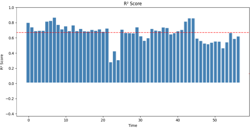
Augmented Samples: 20
