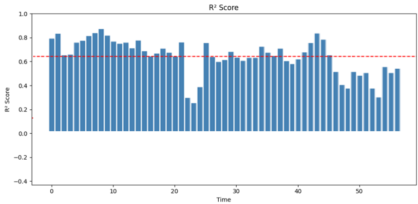
2 masking
