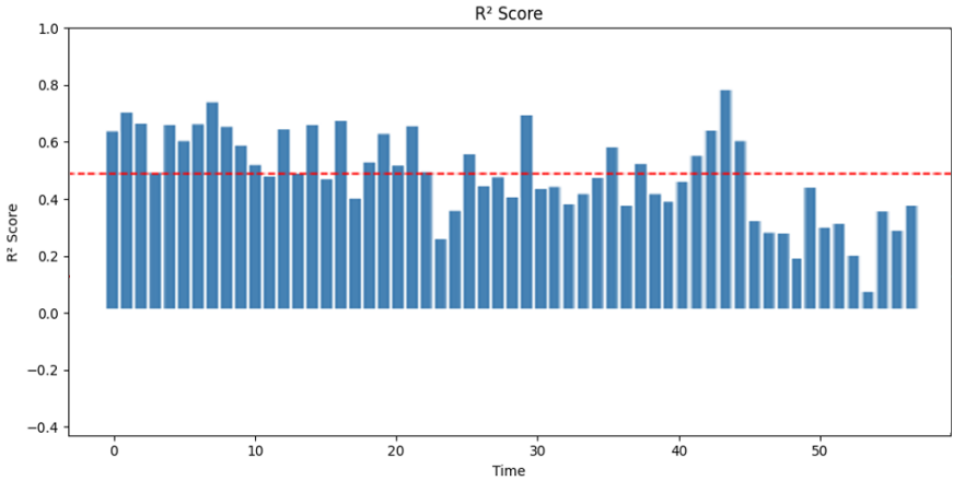
Augmented Samples: 10
